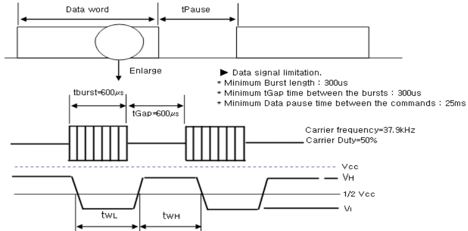
② Fig.2 Application Circuit
