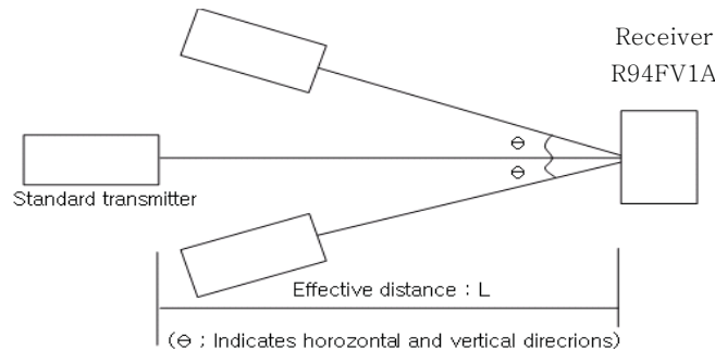
③ Fig.3 Test Condition of Arrival Distance
